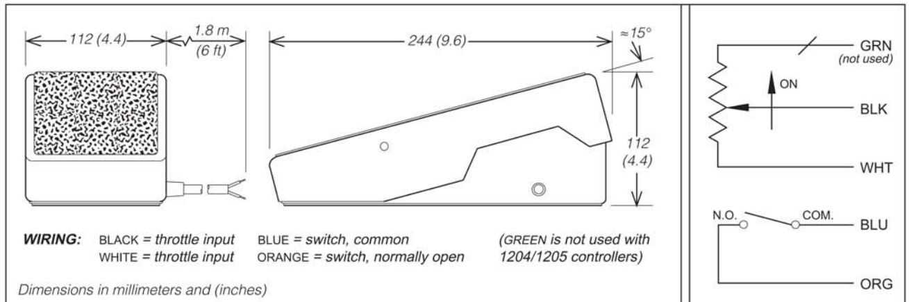
Fig. 4 Curtis PMC footpedal FP-2.
