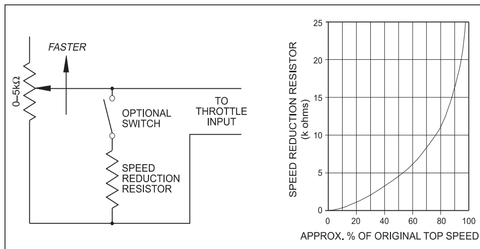
Fig. 13 Reduced speed operation (with standard 0–5kΩ pot).
